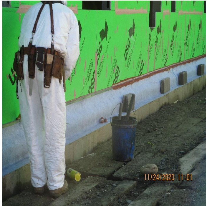
CAULKING ABOVE THROUGH-WALL FLASHING
